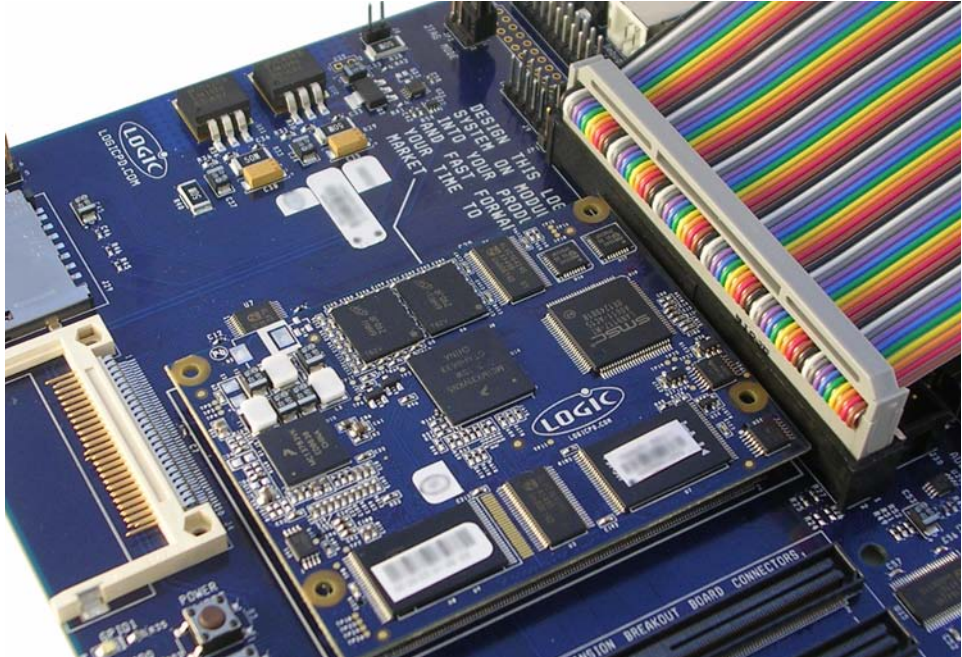
Figure 3.4 – LV-baseboard Ribbon Cable Connection
