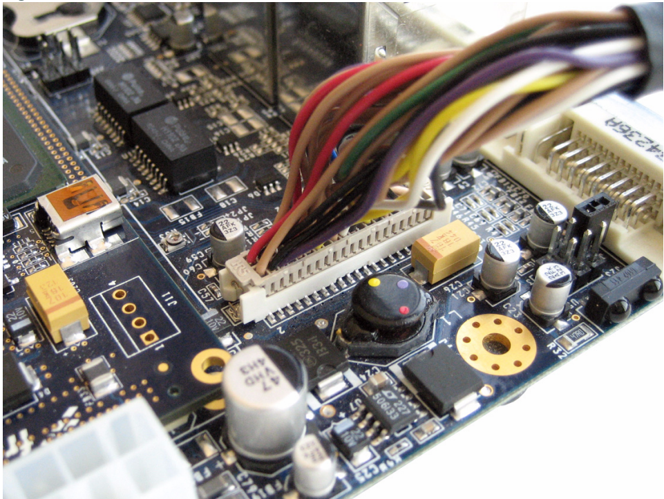
Figure 3.5 – ColdFire EVB Baseboard Cable Connection
