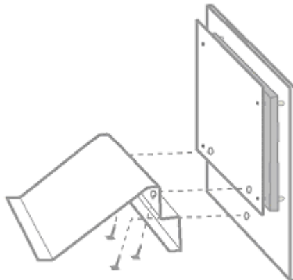
Figure 3.2 – 12.1” Display Kit Assembly
