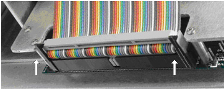
Figure 3.7 – Lock the Connector Latches in the Upright Position
