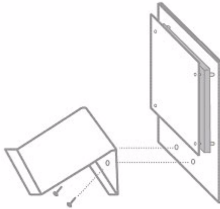
Figure 3.1 – 3.6” and 6.4” Display Kit Assembly
